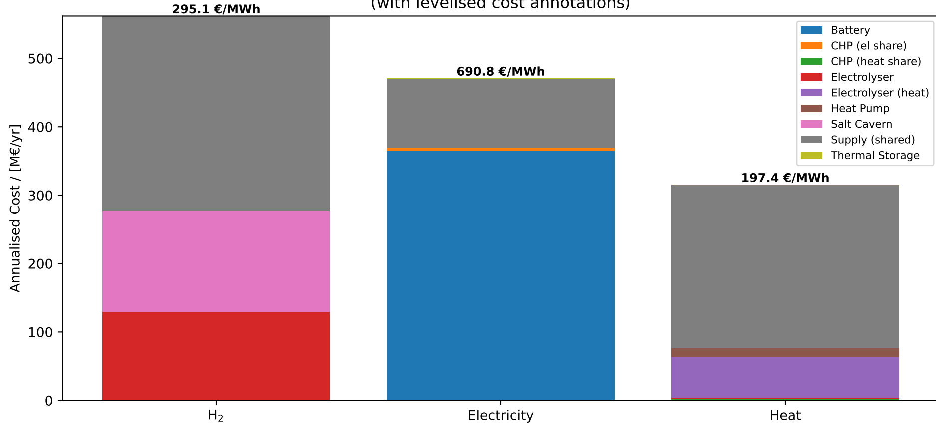
Cost Attribution by Energy Carrier (with levelised cost annotations)
